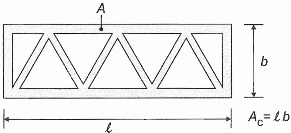
Figure 7.37 — Definition of solidity ratio \phi
